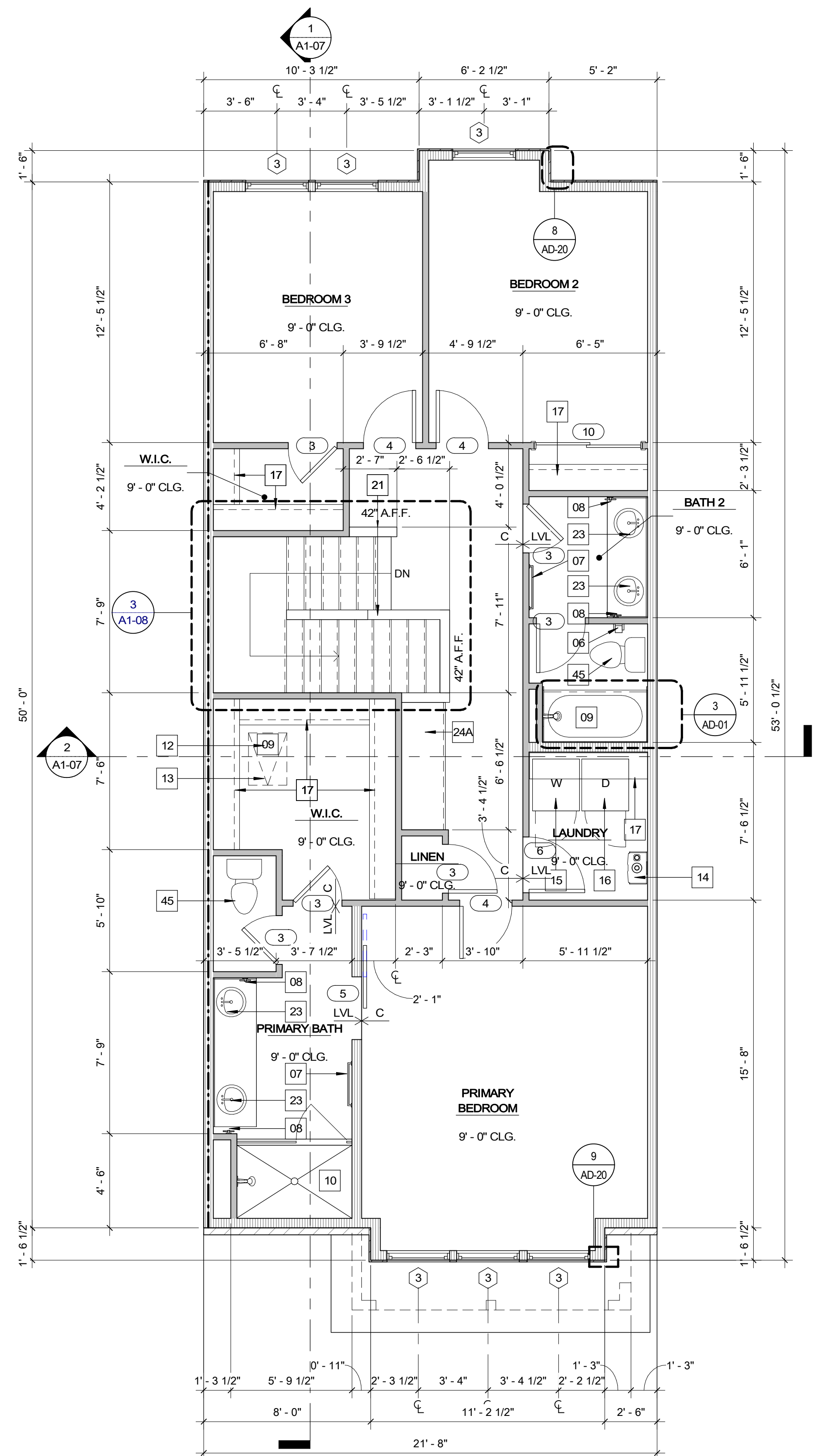
TH - STYLE 'B' PARTIAL FLOOR PLAN - LEVEL 2
